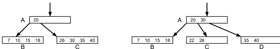
Fig. 4.44. Insertion of key 22 in B-tree
